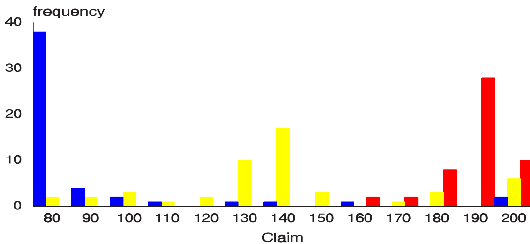
Figure 1. Claim frequencies in a traveler's dilemma with R = 50 (blue), R = 25 (yellow), and R = 10 (red).
