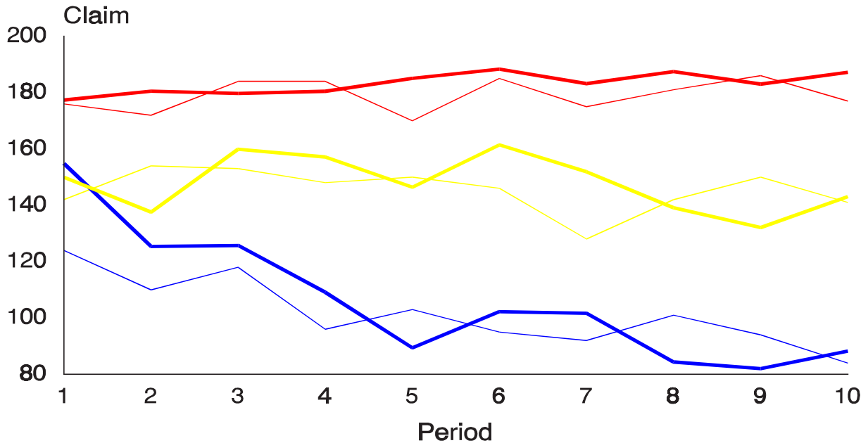
Figure 3. Adjustment patterns in the traveler's dilemma: human data (thick lines) and simulated Bayesian learning (thin lines), by color-coded treatments.
