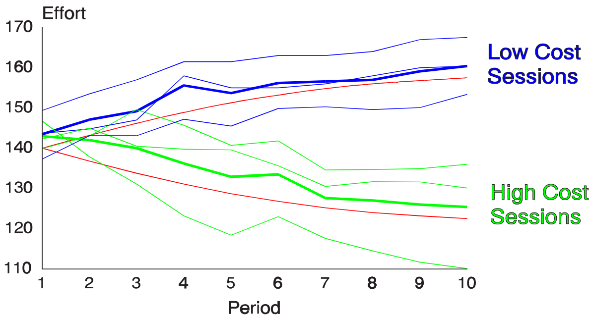
Figure 2. The coordination game: data averages (blue and green lines), and evolutionary predictions (red lines)
