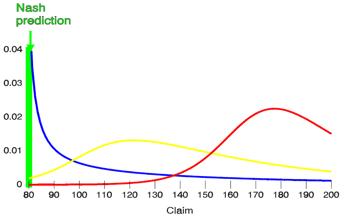
Figure 4. Logit equilibrium densities for the traveler's dilemma, with R = 50 (blue), R = 25 (yellow) and R = 10 (red).
